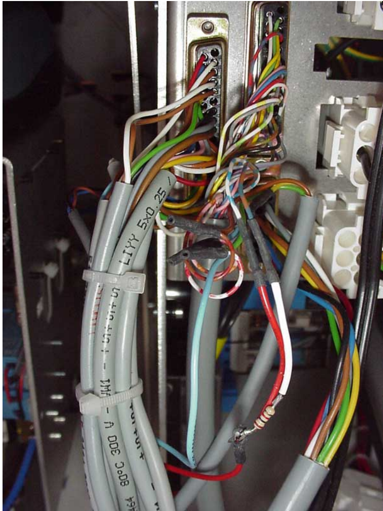
BCR Power Cabling
