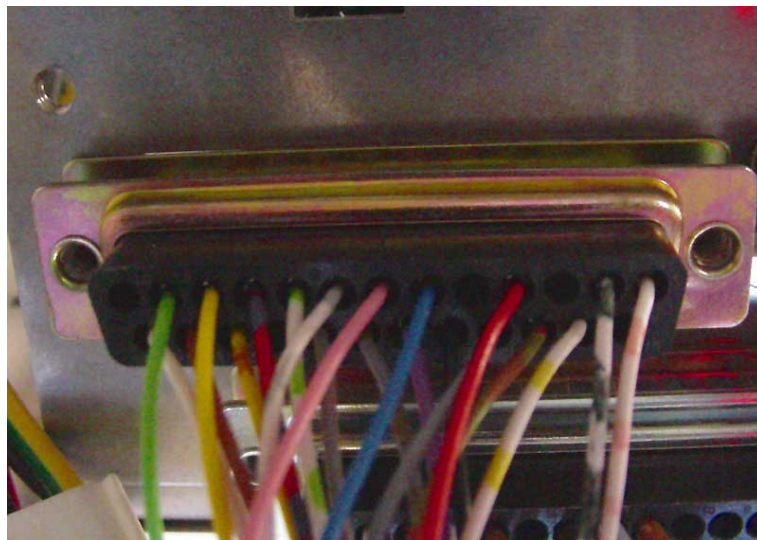
25-Pin D-SUB Handler
